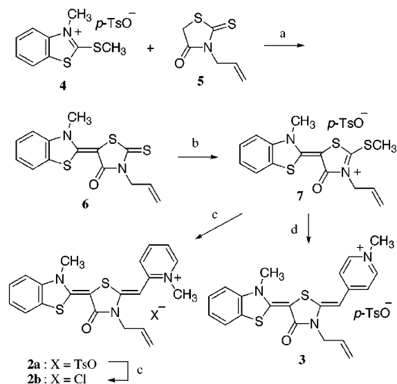
Figure 1. General formula of the rhodacyanine dye.
