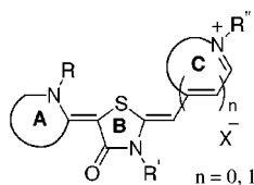
Figure 1. General formula of the rhodacyanine dye.
